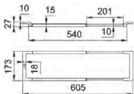
Sistem telescopic
